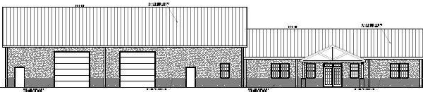
1 FRONT ELEVATION 1/4" = 1'-0"
